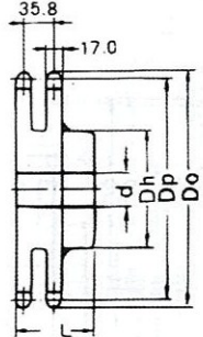
DUPLEX BW TYPE
