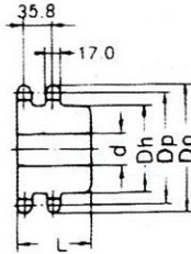
DUPLEX B TYPE
